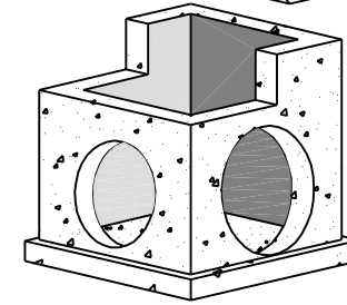
TYPE-18 CURB INLET
